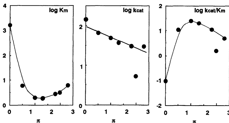
Fig. 1. The relationship between the hydrophobicity of the alkyl group and K_m , k_{cat} , and k_{cat}/K_m for the catalysis of alkylmalate by IPMDH replotted from the values in Table I. Energies are in kcal/mol. The \pi values are the Hansch constants for the alkyl substituents [15].
